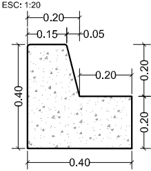
DETALLE BROCAL
