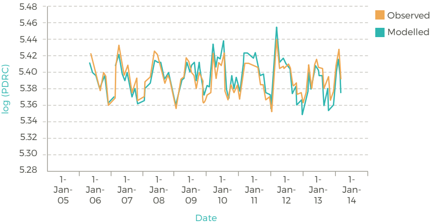
Figure 1 Comparison of predicted and observed water demand
